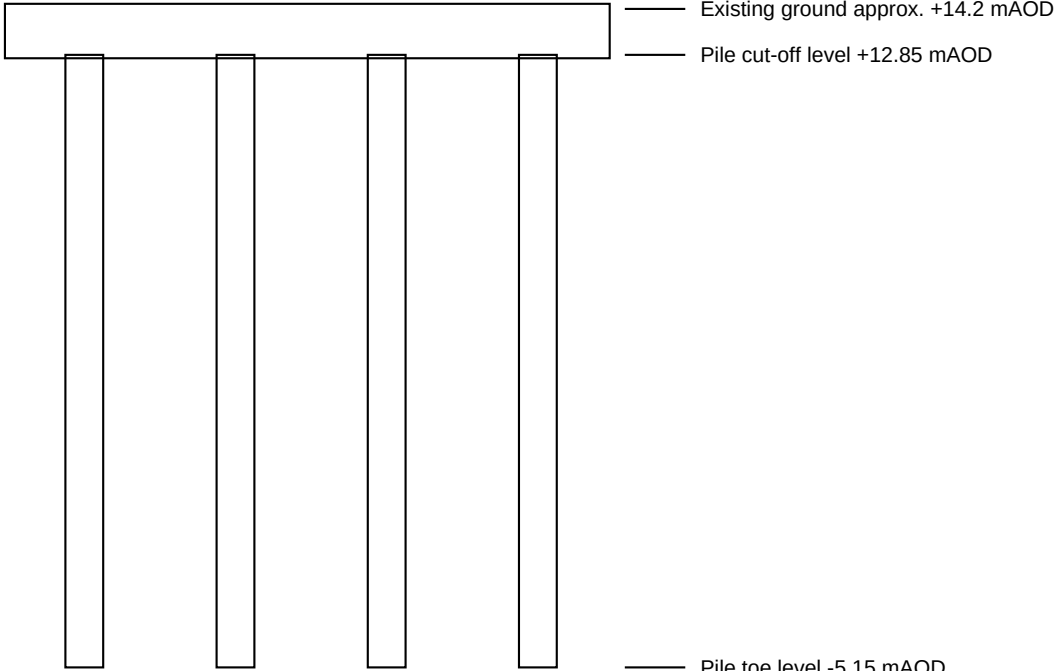
8 No. 900 mm dia. bored piles, 18.0 m long
